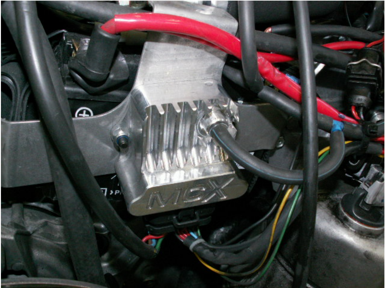
The MCX EFI-box controls both the fuel delivery in the external injectors and the turbo pressure to prevent the power to drop at higher altitudes.
