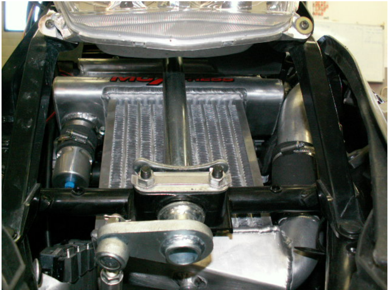
The intercooler is placed in front of the engine. The extra injectors are integrated in the plenum. A blow off valve is installed on the plenum.
